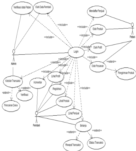
Gambar 3. Diagram UseCase
