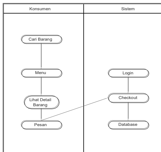
Gambar 4.4 Activity Diagram
