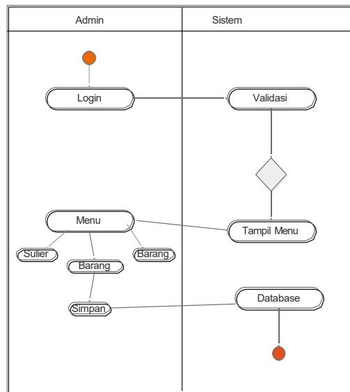
Gambar 4.3. Activity Diagram
